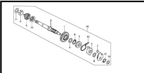
E-15-2 ARRANQUE 2008
