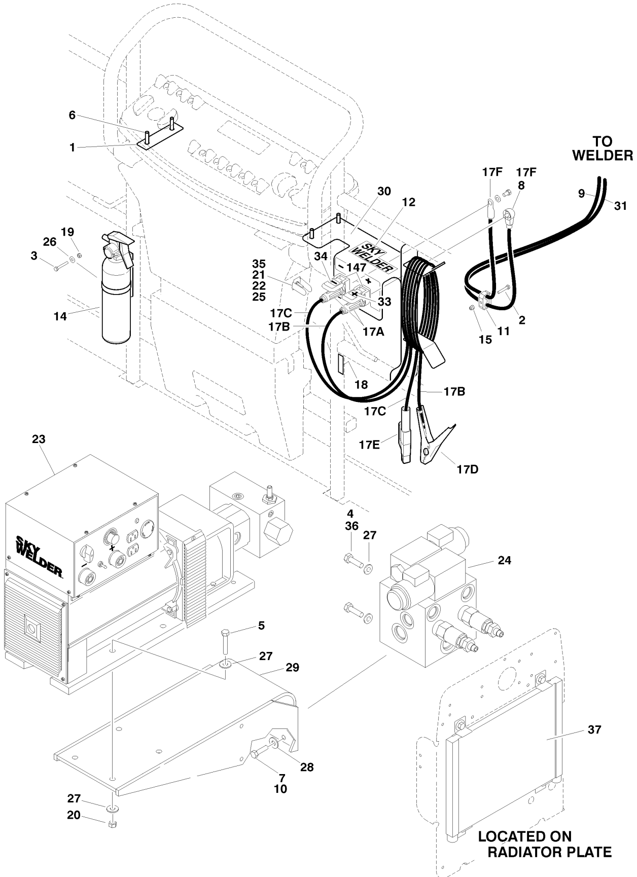
FIGURE 10-2. SKY WELDER INSTALLATION
