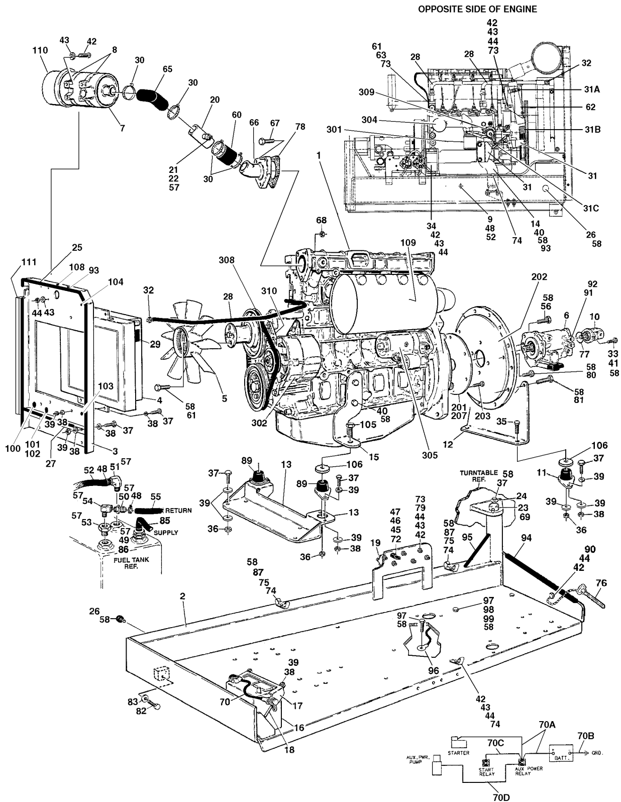
FIGURE 2-11. DEUTZ ENGINE INSTALLATION - 4CYL (WITHOUT ADE)
