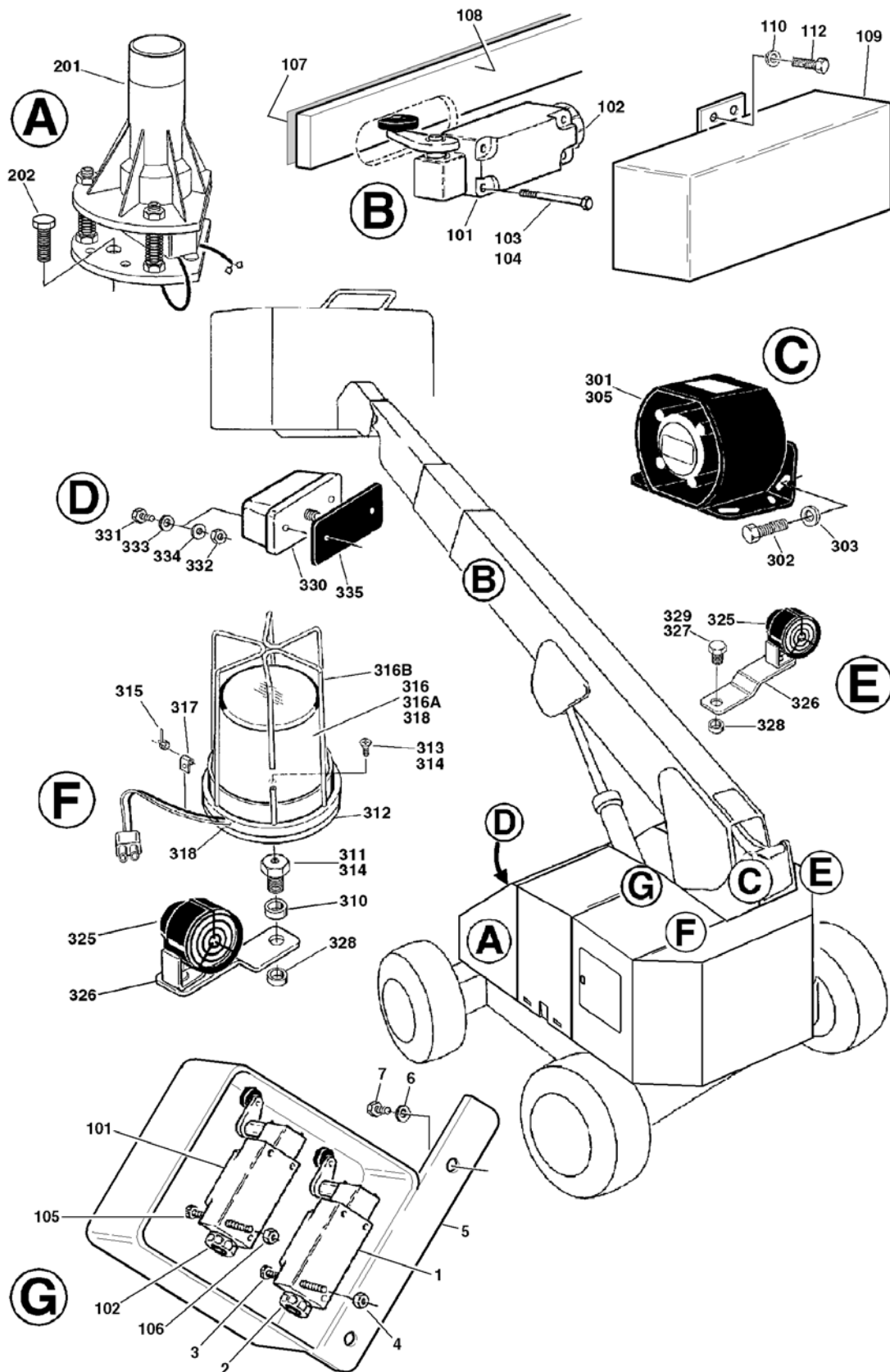
FIGURE 2-28. ELECTRICAL OPTIONS INSTALLATION (TURNTABLE MOUNTED)
