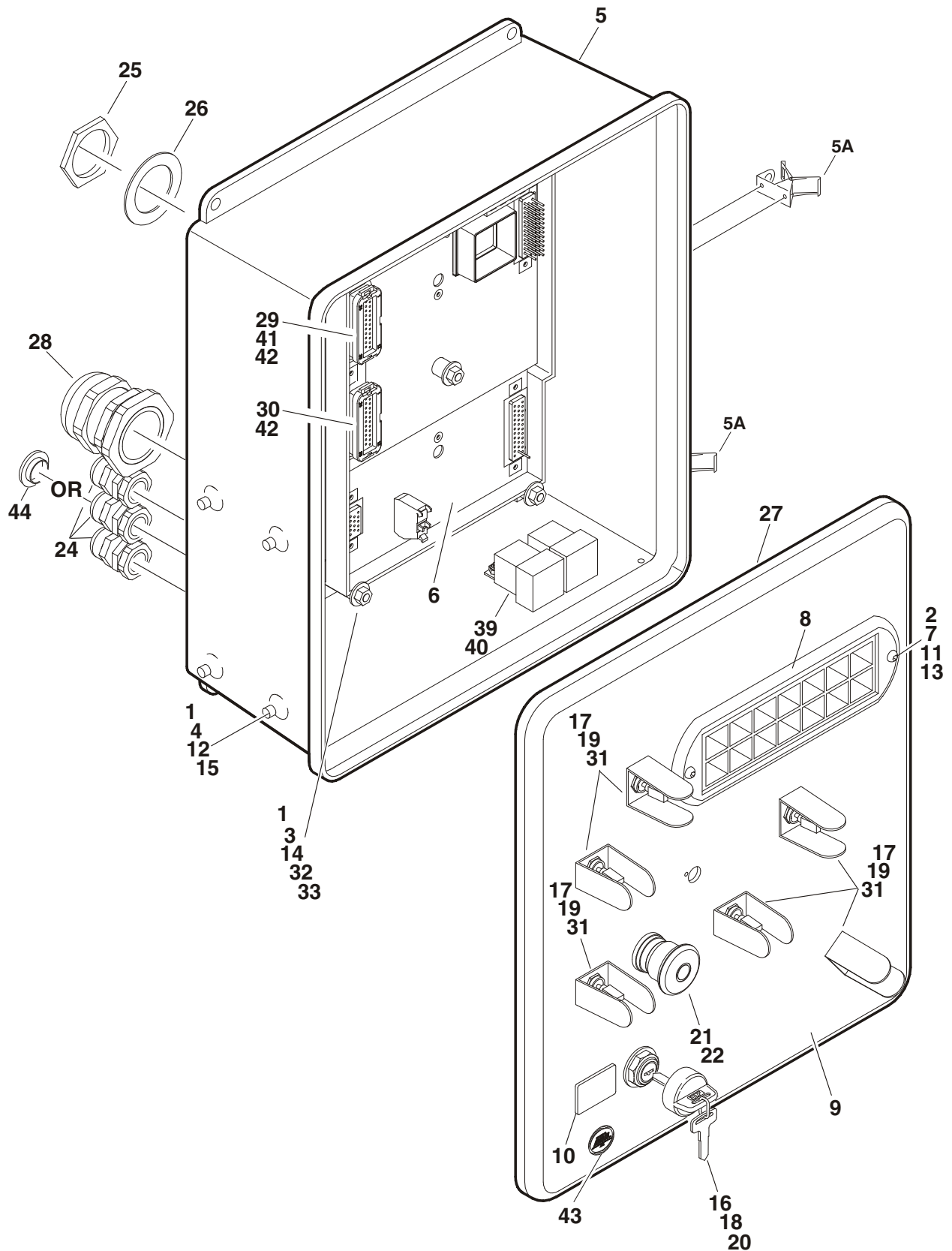
FIGURE 2-27. GROUND CONTROL BOX ASSEMBLIES (ADE SYSTEM) (S/N 62137 TO PRESENT)
