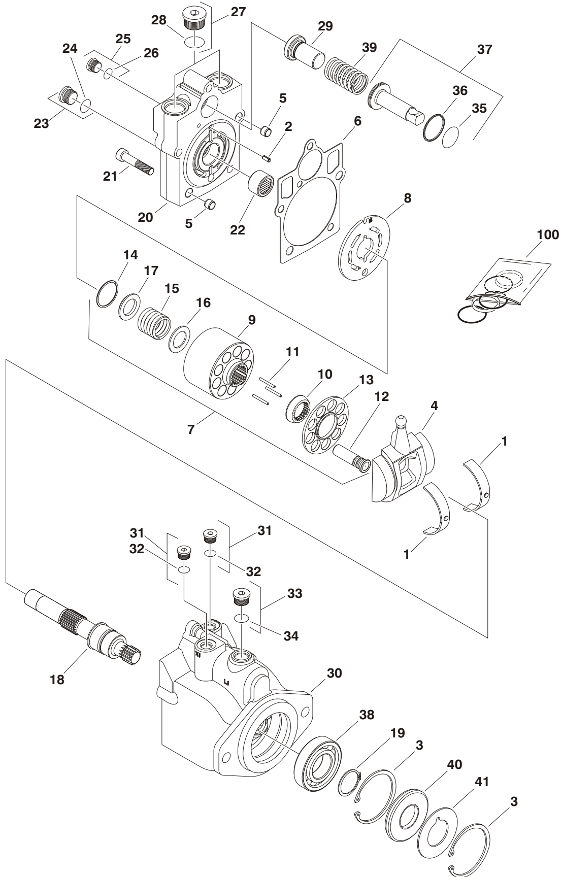
FIGURE 1-11. DRIVE MOTOR ASSEMBLY (5 BOLT ASSEMBLY) (S/N 98765 TO PRESENT)
