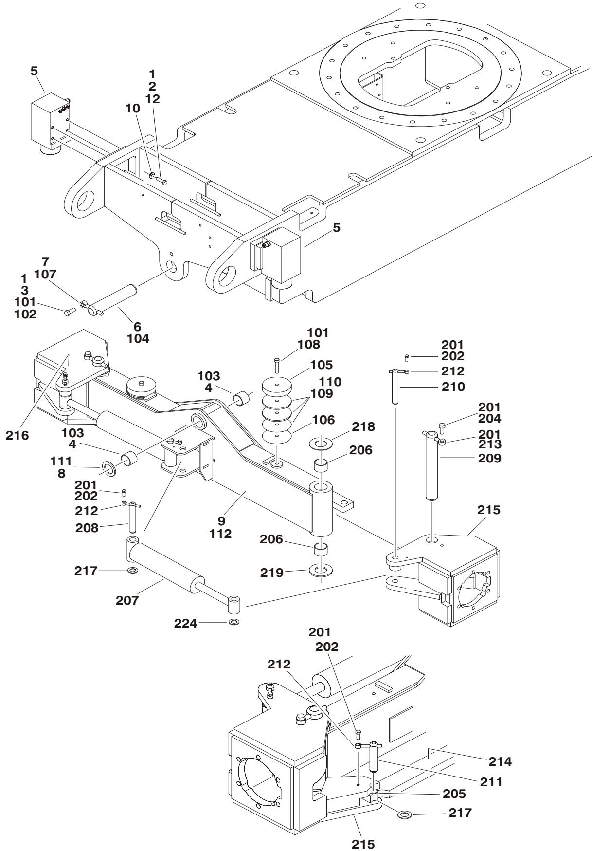
FIGURE 1-2. 4WD FRONT AXLE AND STEERING INSTALLATIONS (S/N 85132 TO PRESENT)
