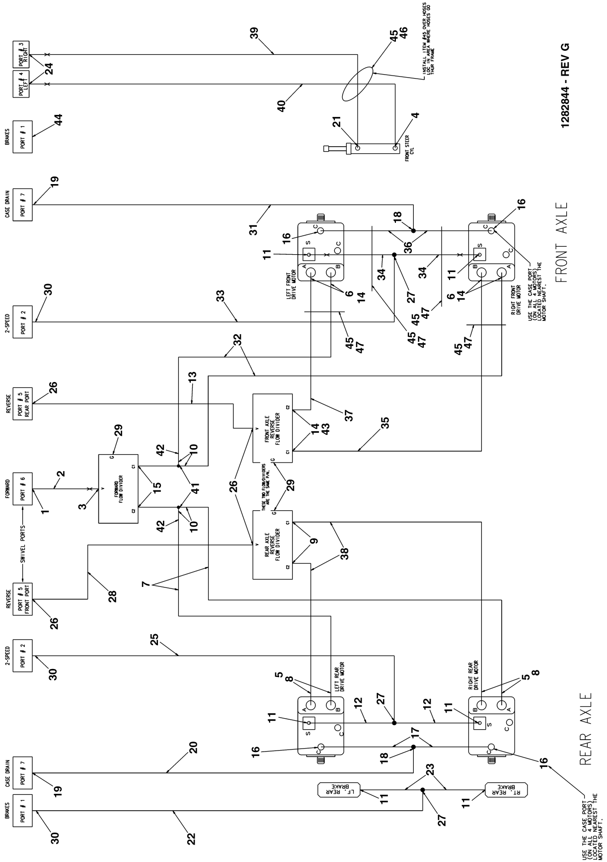
FIGURE 6-1. HYDRAULIC DIAGRAM - DRIVE & STEER (PRIOR TO S/N 85132)
