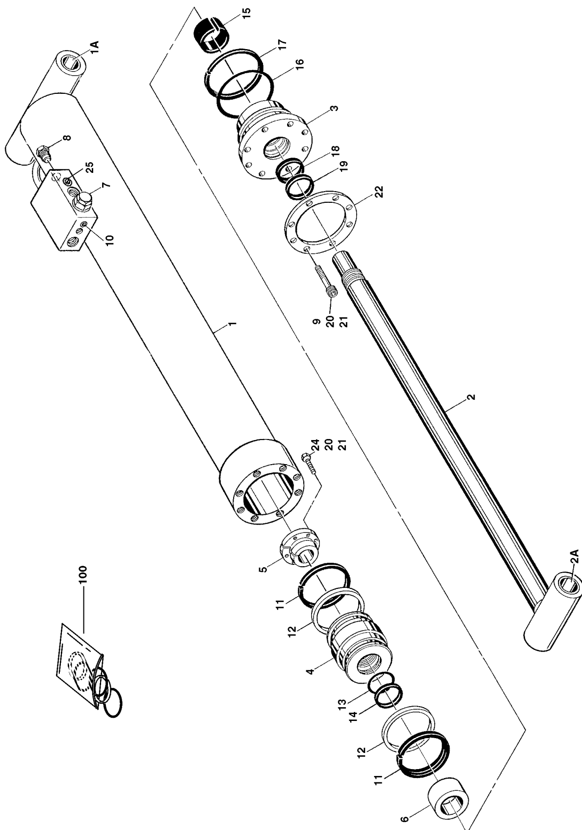
FIGURE 5-4. LIFT (BOOM) CYLINDER ASSEMBLY
