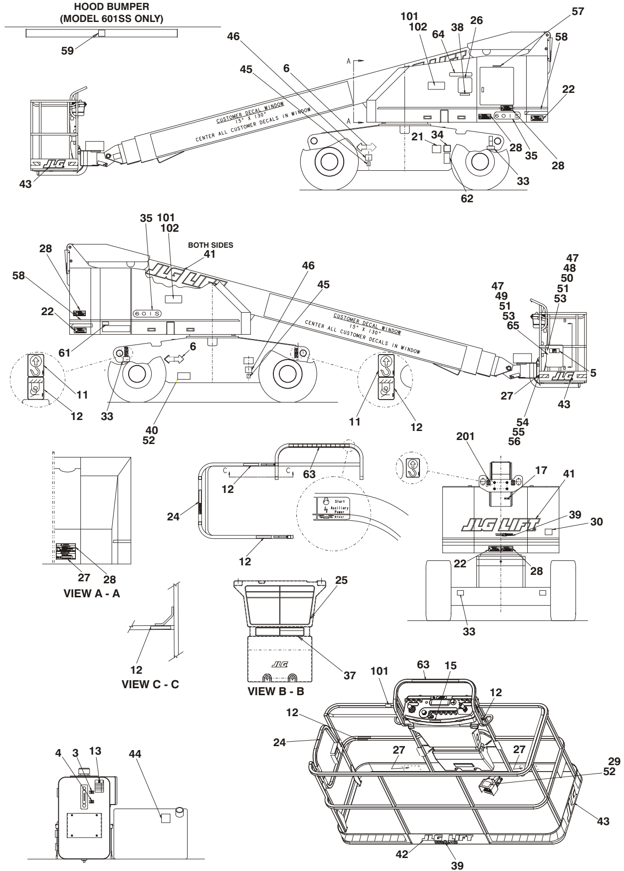
FIGURE 8-4. DECAL INSTALLATION (COUNTRY SPEC) (S/N 87744 TO PRESENT)
