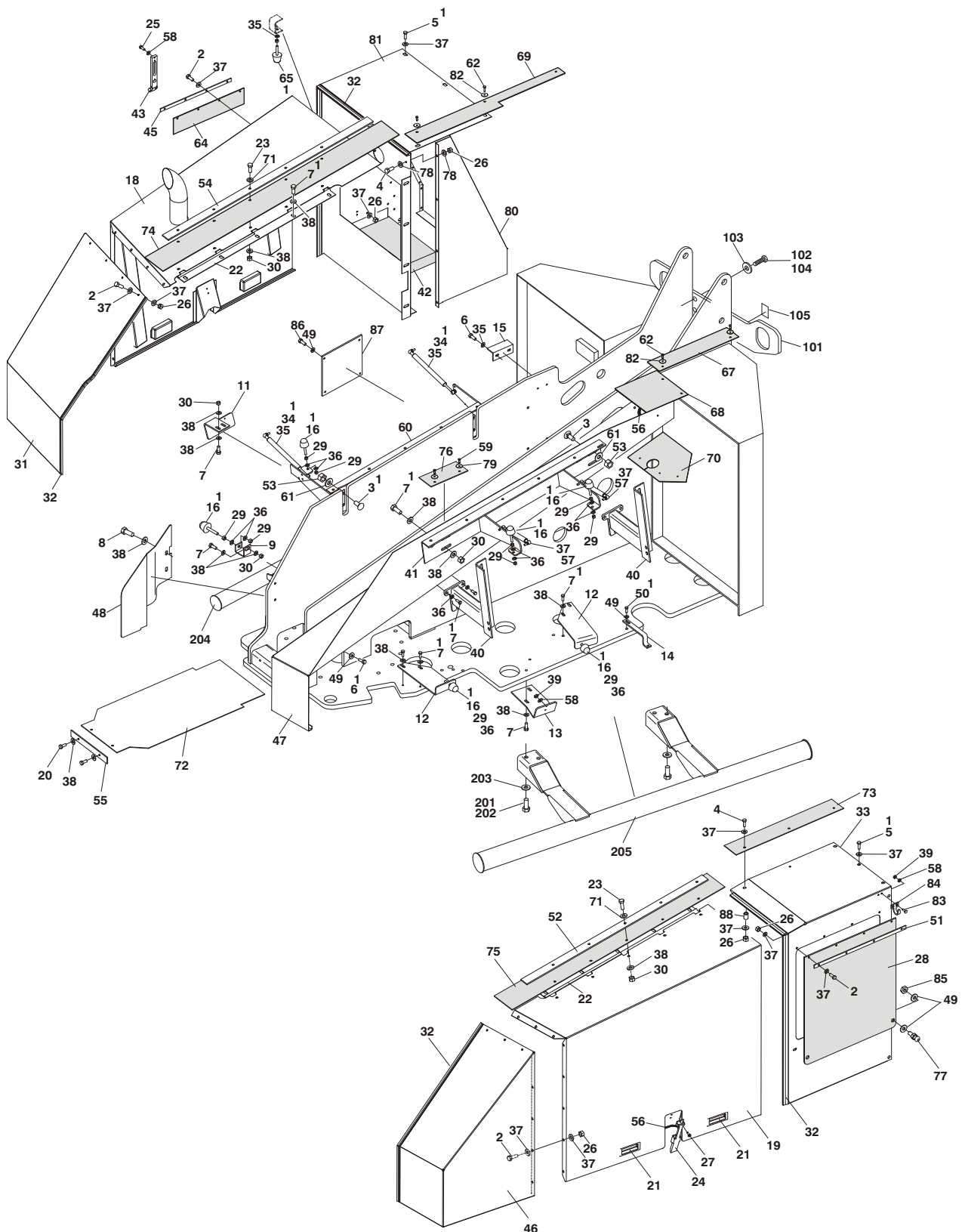
FIGURE 2-30. HOODS INSTALLATION - MODEL 601S WITH A "ENHANCED HOSTILE ENVIRONMENT PACKAGE")
