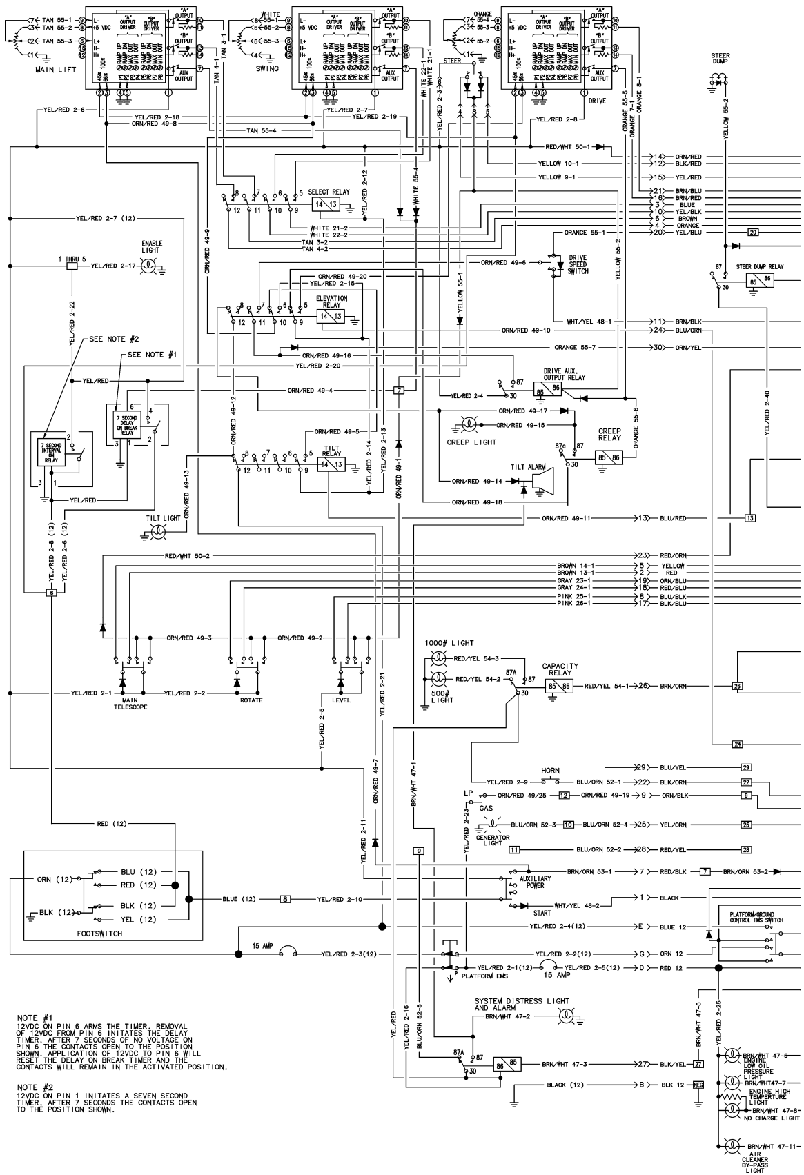
FIGURE 7-4. ELECTRICAL SCHEMATIC - FORD ENGINE MACHINES (S/N 58209 TO S/N 62137)
