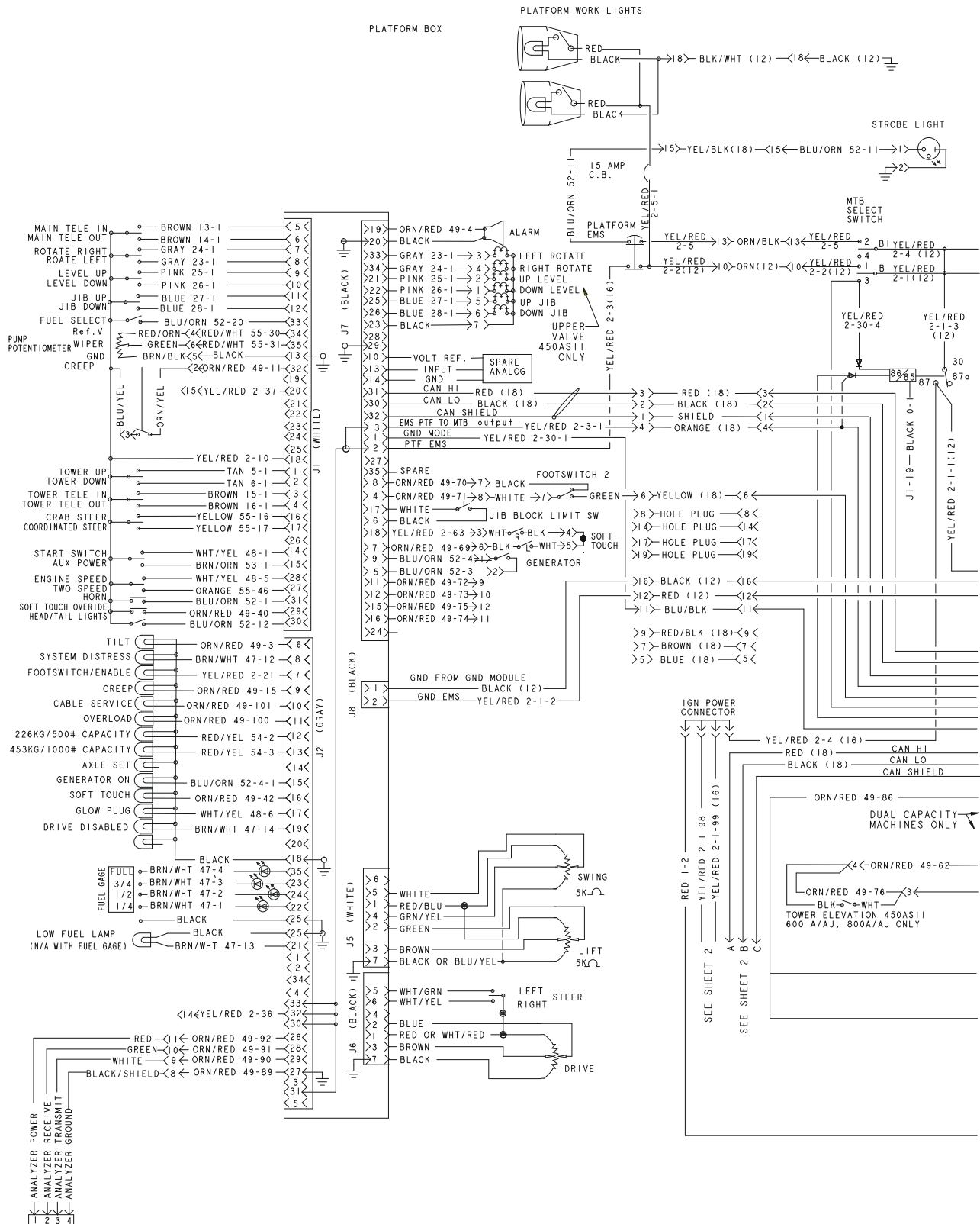
FIGURE 7-7. ELECTRICAL SCHEMATIC - DEUTZ TIER 2 (S/N 99060 TO PRESENT)
