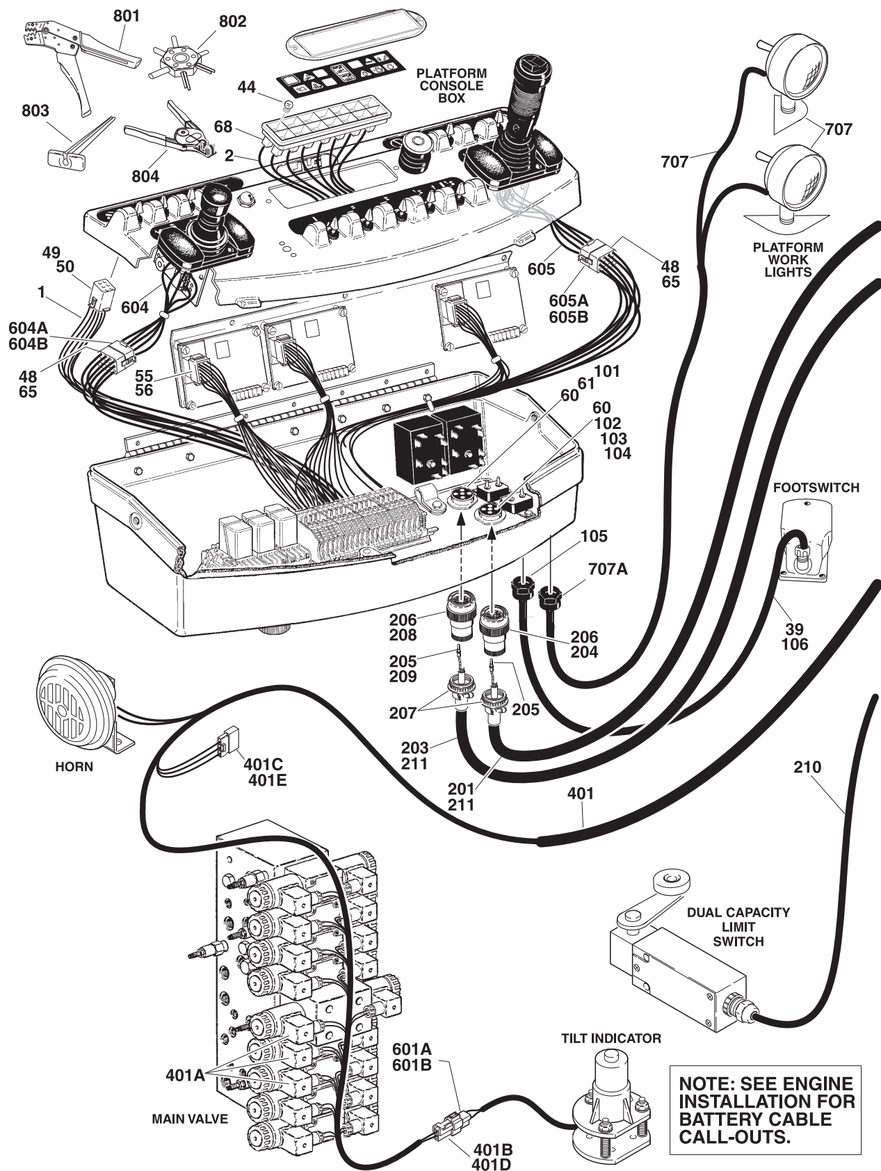
FIGURE 7-8. HARNESS COMPONENTS INSTALLATION (PRIOR TO S/N 62137)
