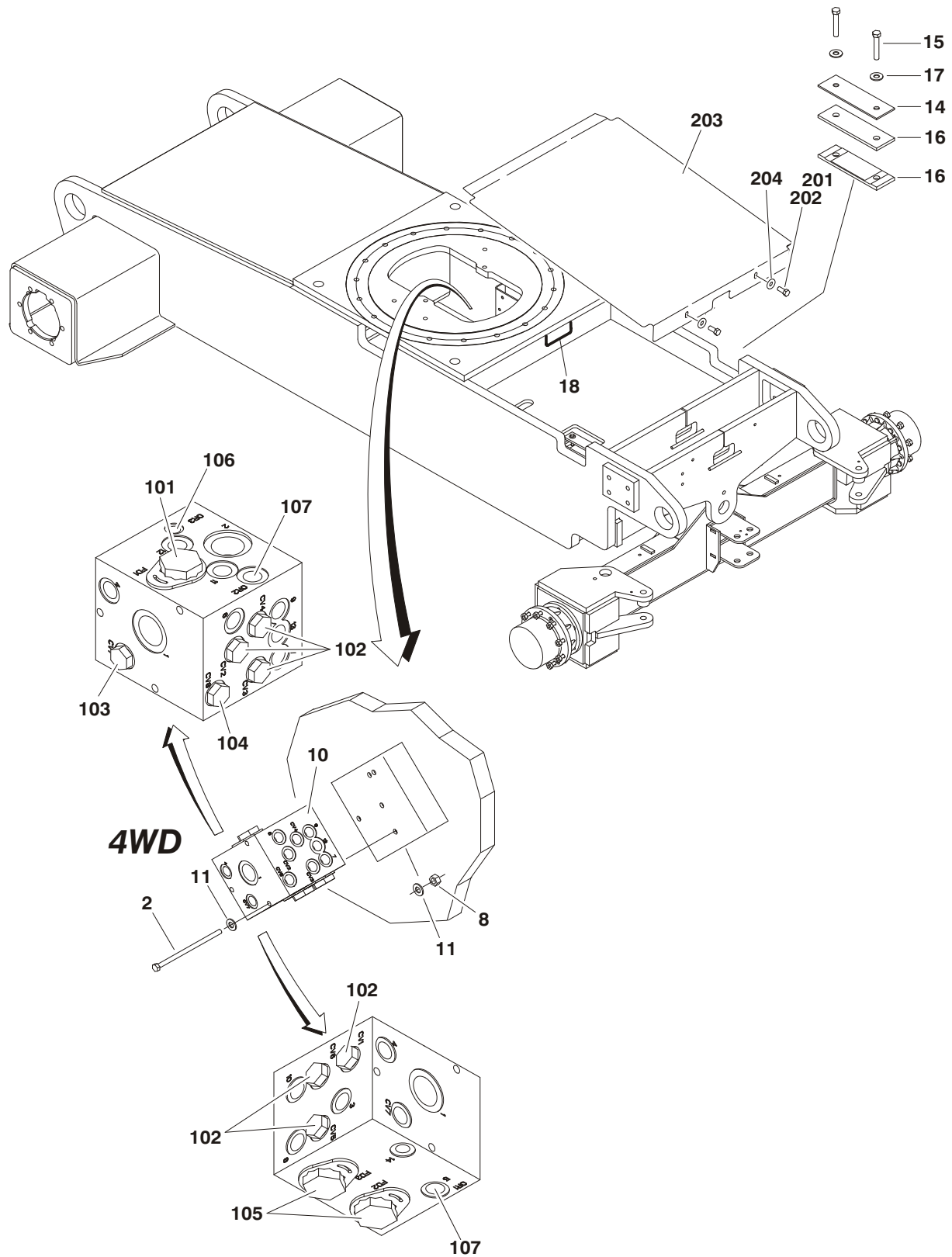
FIGURE 1-13. DRIVE VALVES & SHIELDS INSTALLATION (FRAME MOUNTED) (S/N 85132 TO PRESENT)
