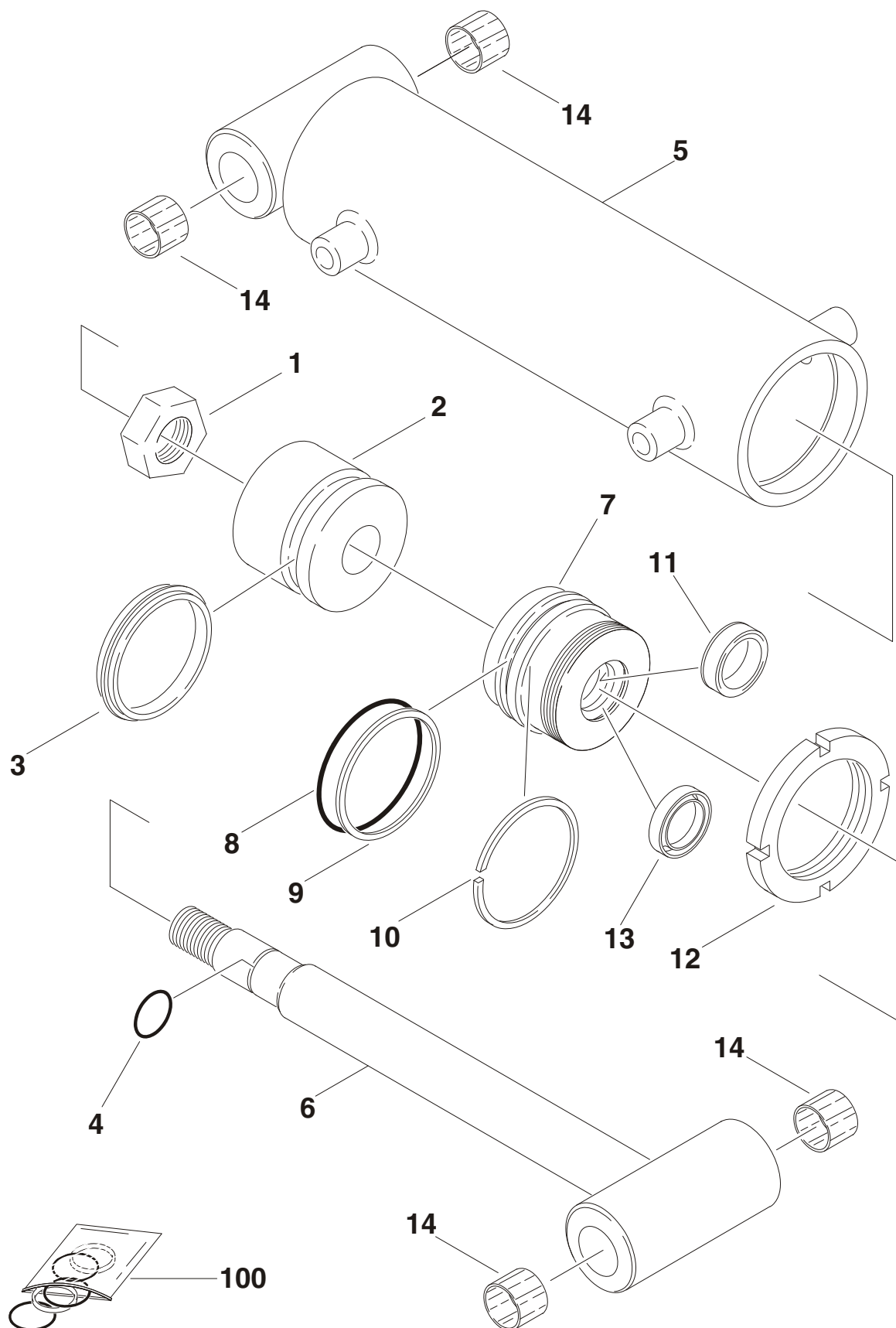
FIGURE 5-7. STEER CYLINDER ASSEMBLY (S/N 85132 TO PRESENT)
