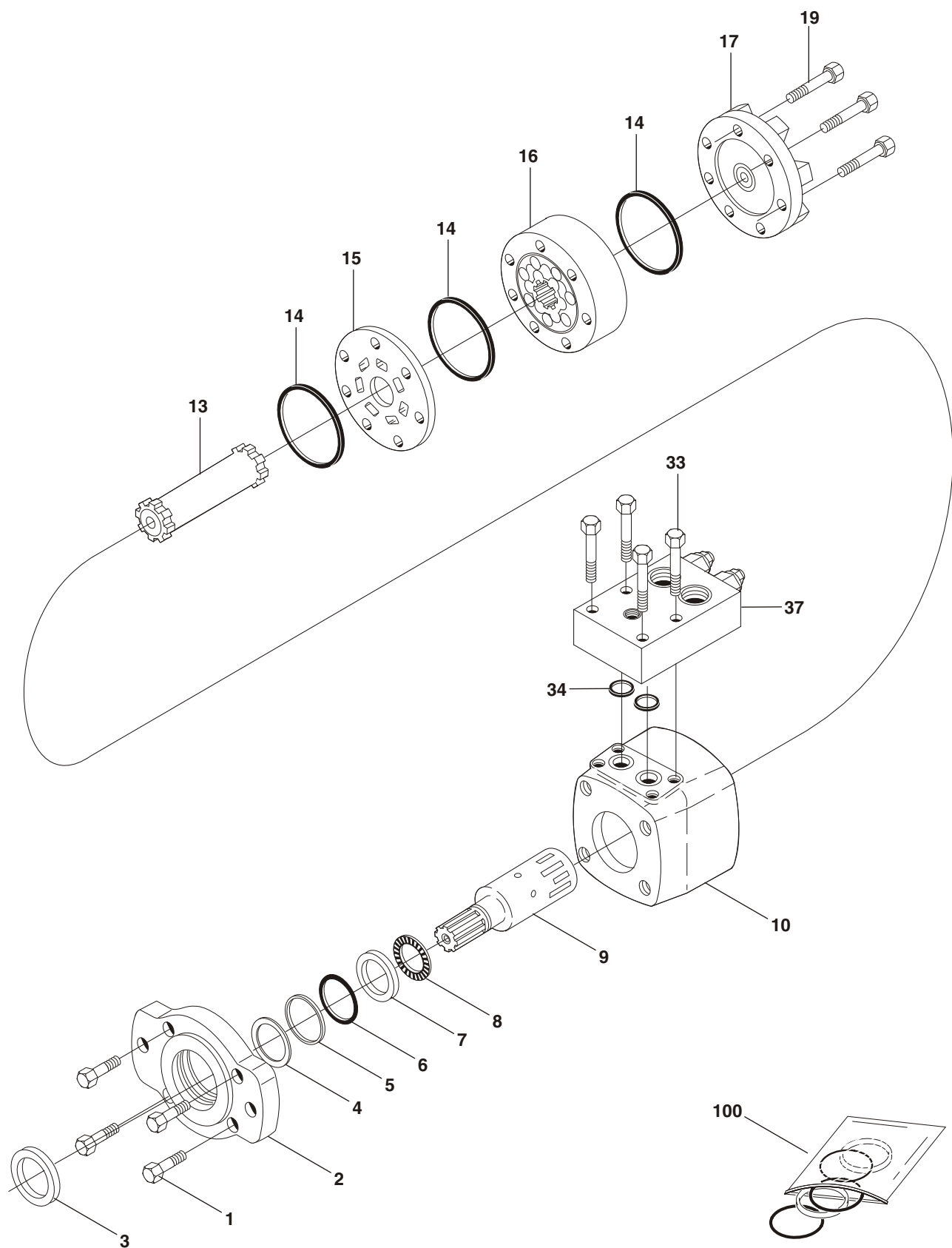
FIGURE 2-8. SWING MOTOR ASSEMBLY
