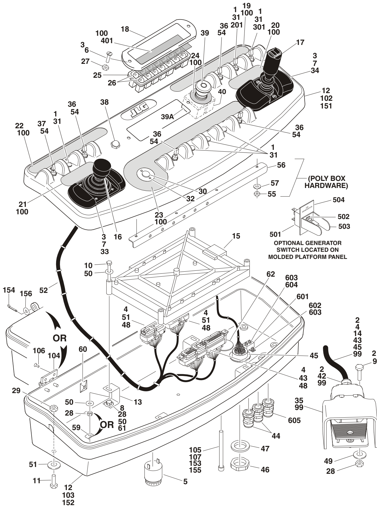
FIGURE 4-4. PLATFORM CONSOLE BOX ASSEMBLES - WITH ADE SYSTEM (S/N 62137 TO PRESENT)
