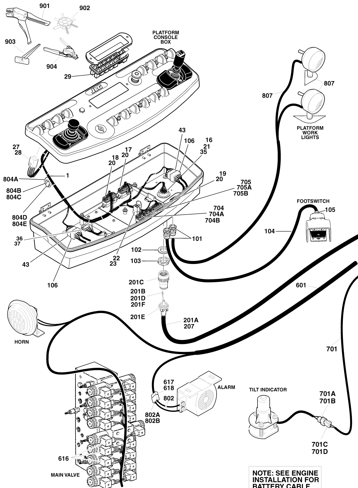
FIGURE 7-9. HARNESS COMPONENTS INSTALLATION (WITH ADE SYSTEM) (S/N 62137 TO S/N 85132)
