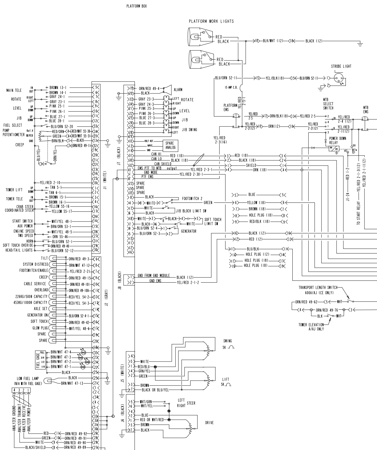
FIGURE 7-5. ELECTRICAL SCHEMATIC - DEUTZ/FORD EFI ENGINE MACHINES (ADE SYSTEM) (W/INTERNAL TILT) (S/N 62137 TO S/N 99060)
