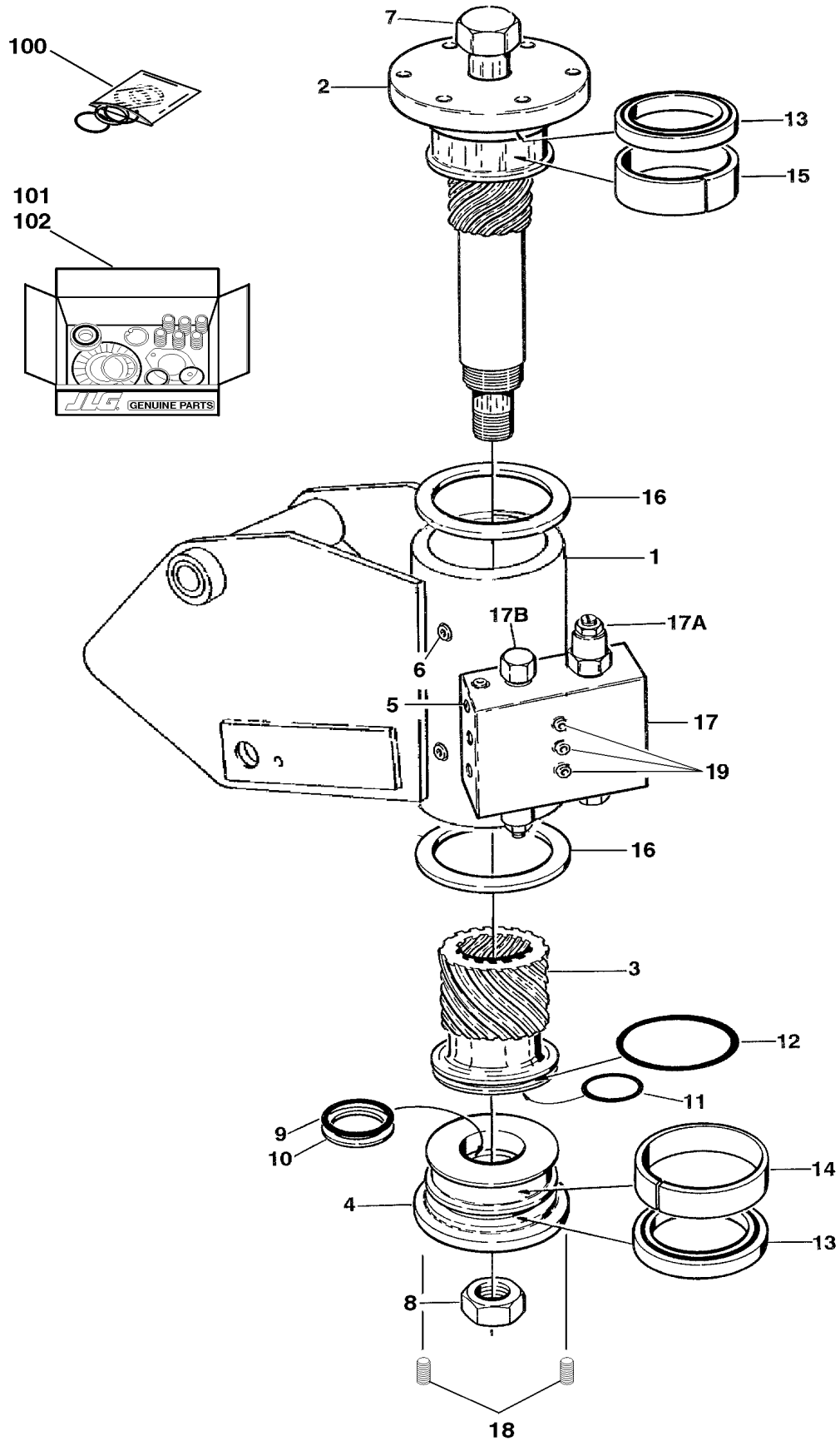
FIGURE 3-3. ROTATOR ASSEMBLY (FRONT ENTRY PLATFORM)
