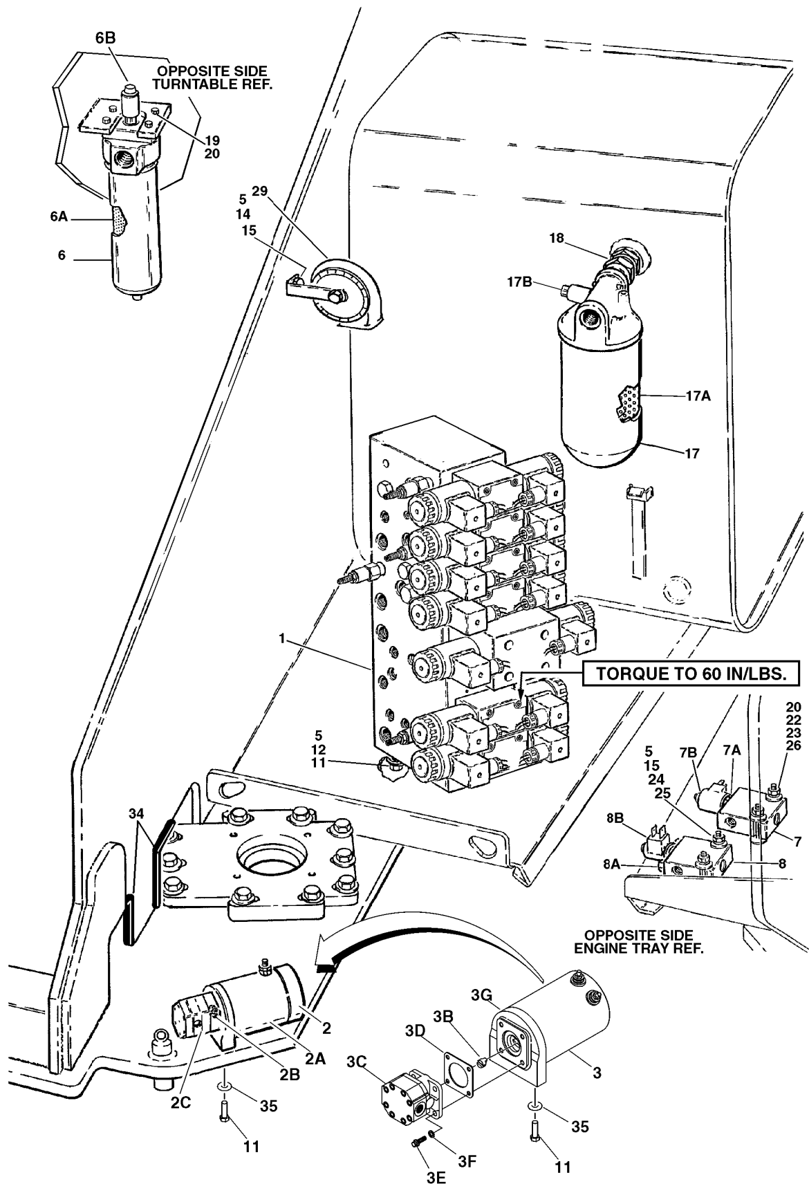
FIGURE 2-1. CONTROL VALVES INSTALLATIONS (PRIOR TO S/N 85132)
