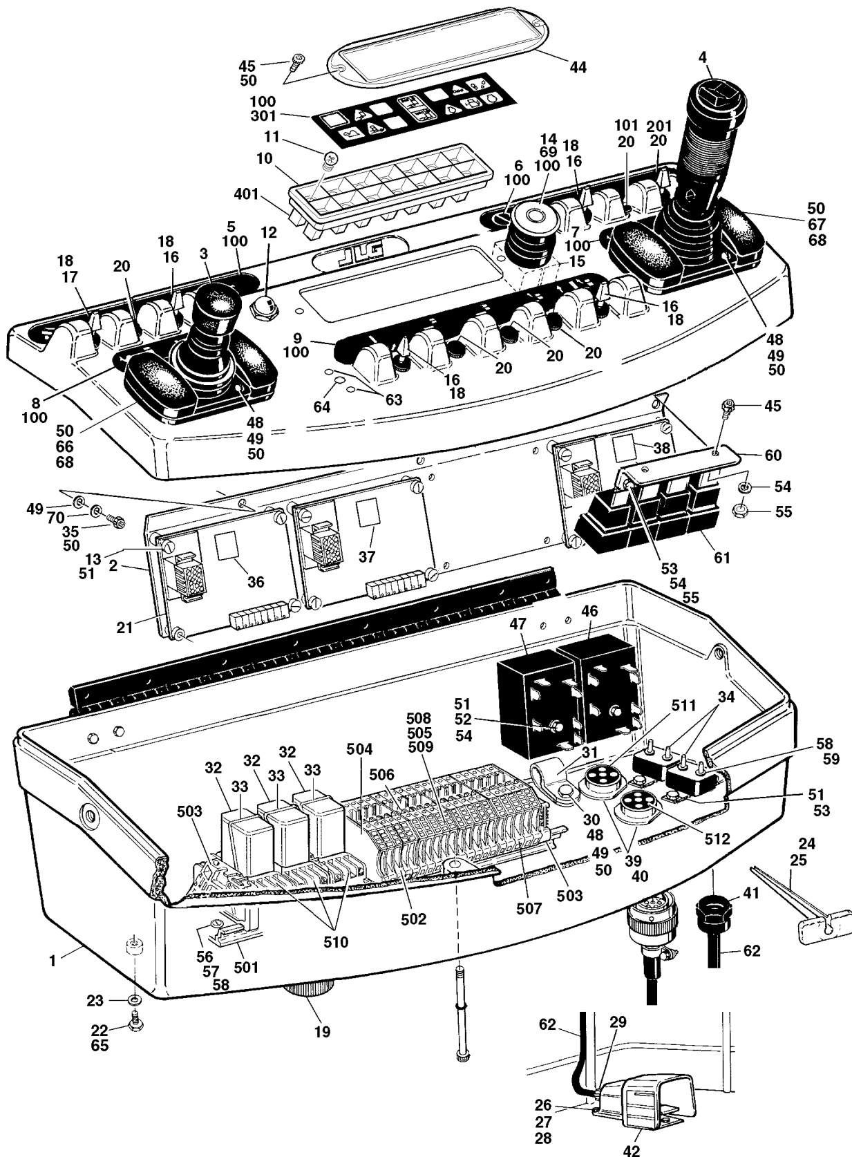
FIGURE 4-3. PLATFORM CONSOLE BOX ASSEMBLIES (PRIOR TO S/N 62137)
