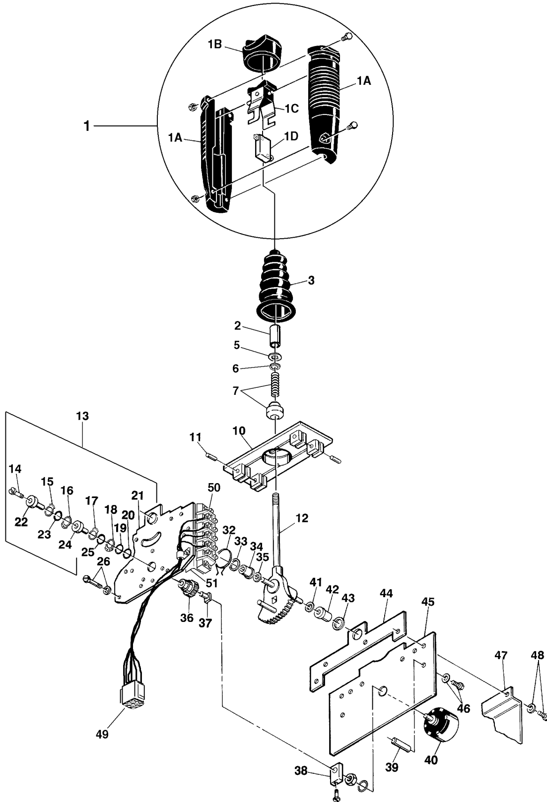
FIGURE 4-8. CONTROLLER ASSEMBLY (DRIVE & STEER) (PRIOR TO S/N 39653)
