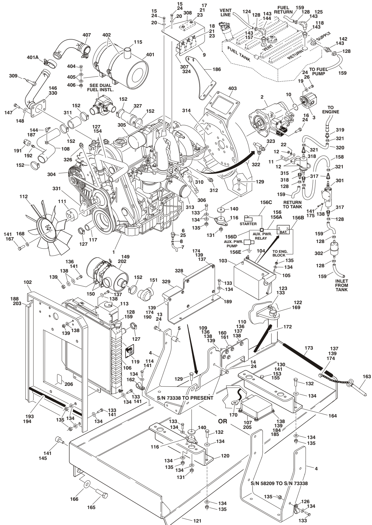
FIGURE 2-15. FORD ENGINE INSTALLATION - LRG425 WITH EFI (S/N 58209 TO PRESENT)
