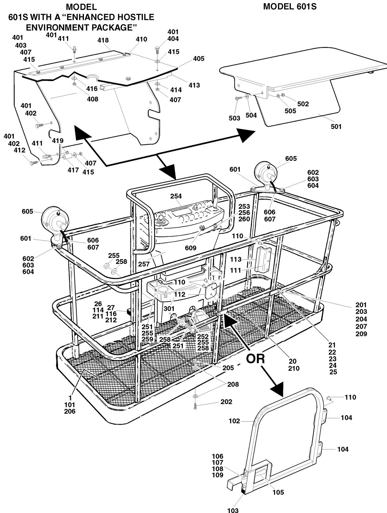
FIGURE 4-1. PLATFORM COMPONENTS INSTALLATION (FRONT ENTRY PLATFORM)
