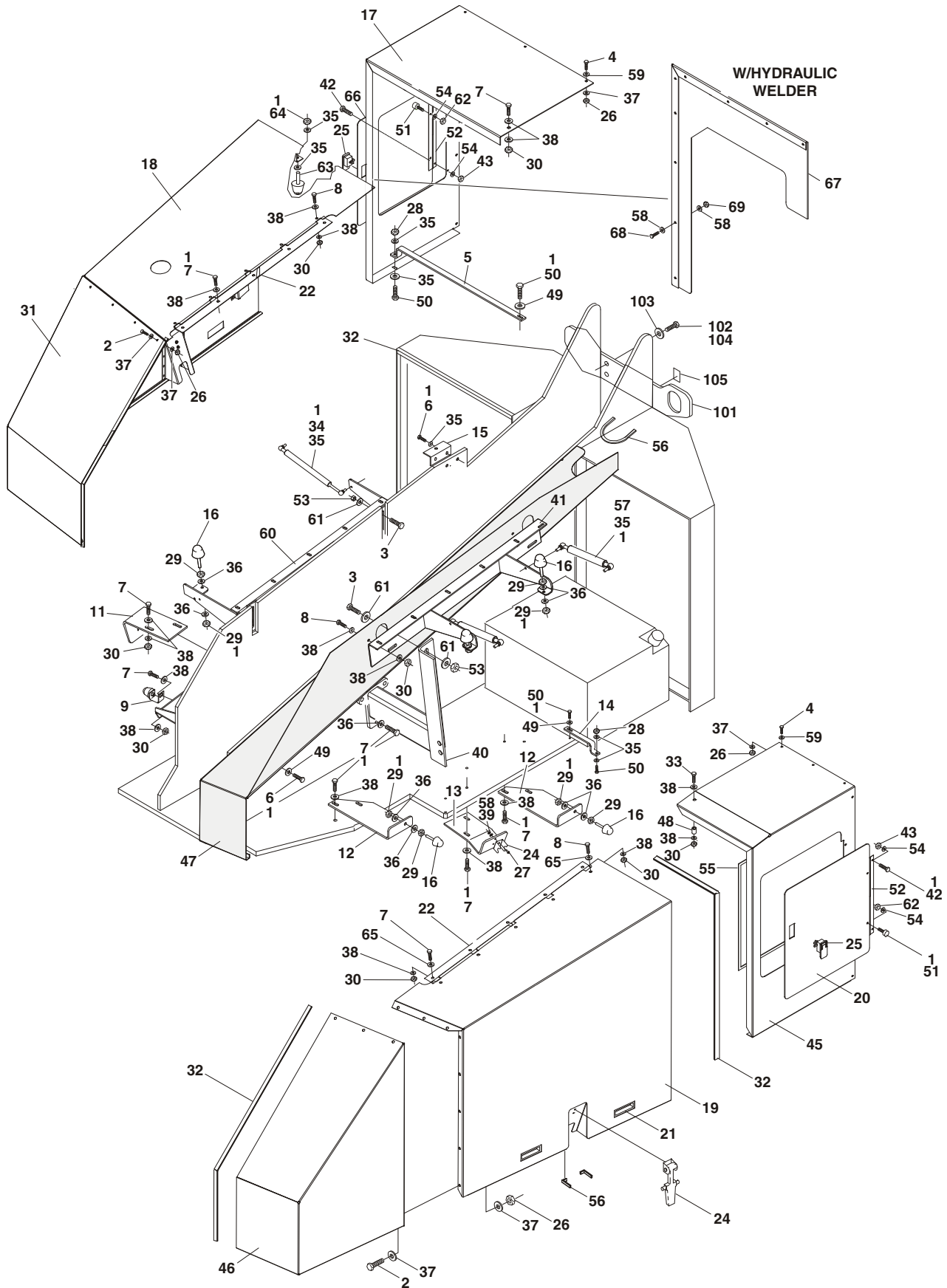
FIGURE 2-29. HOODS INSTALLATION - MODEL 601S
