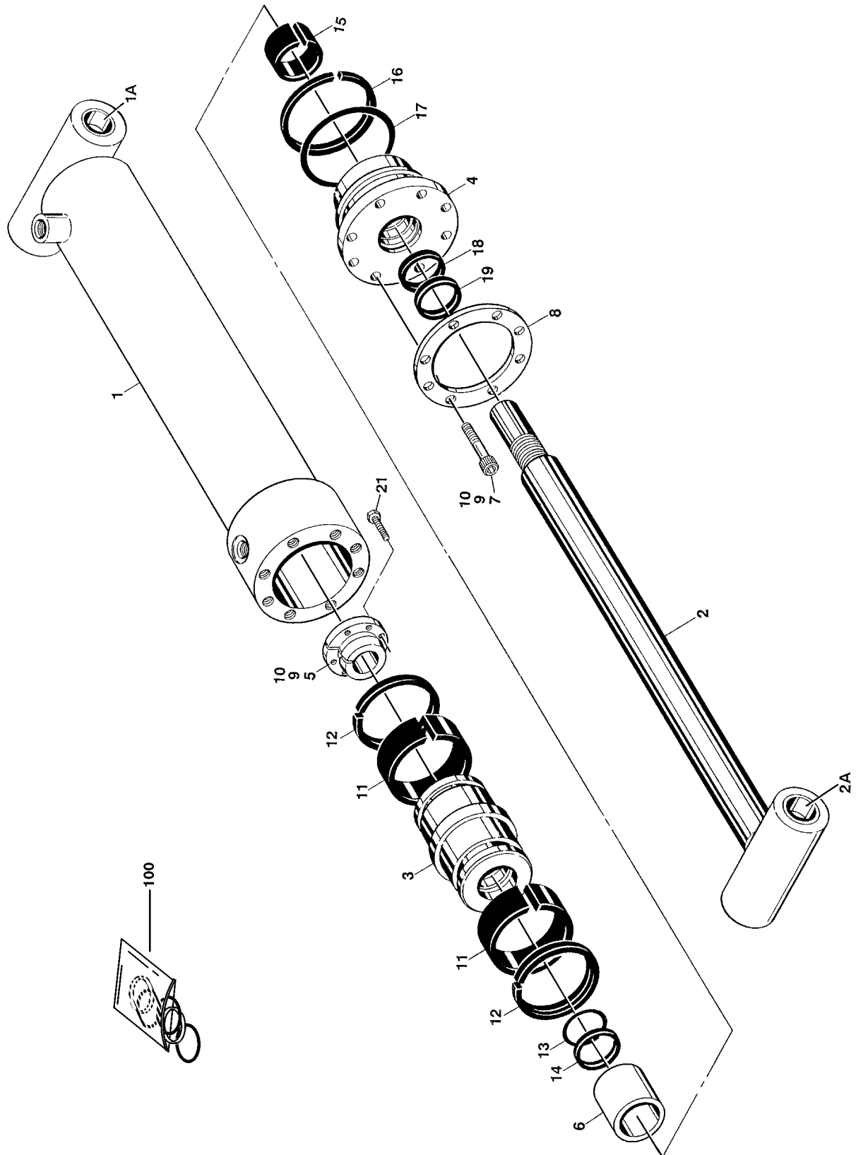
FIGURE 5-5. MASTER CYLINDER ASSEMBLY
