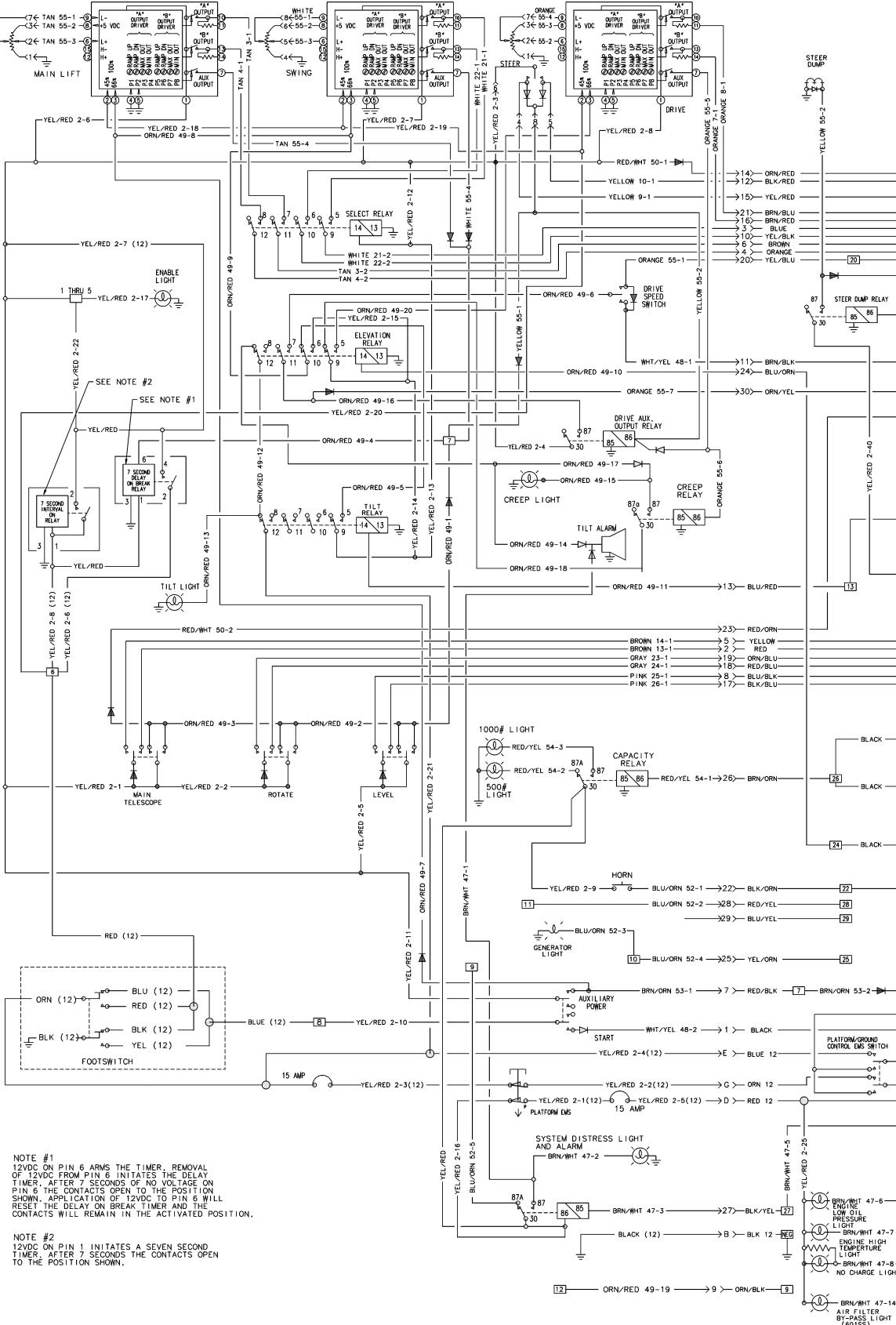
FIGURE 7-2. ELECTRICAL SCHEMATIC - DEUTZ ENGINE MACHINES (PRIOR TO S/N 62137)
