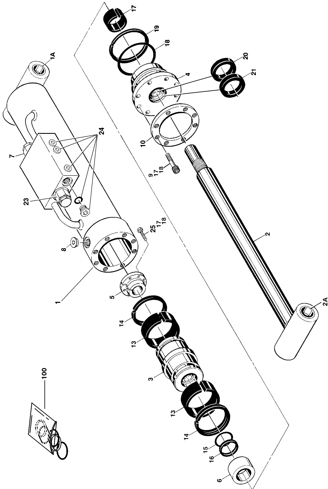
FIGURE 5-3. PLATFORM LEVEL CYLINDER ASSEMBLY
