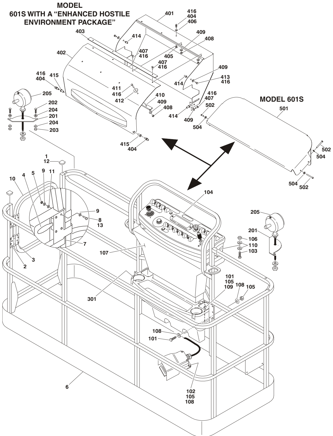
FIGURE 4-2. PLATFORM COMPONENTS INSTALLATION - SIDE ENTRY PLATFORM
