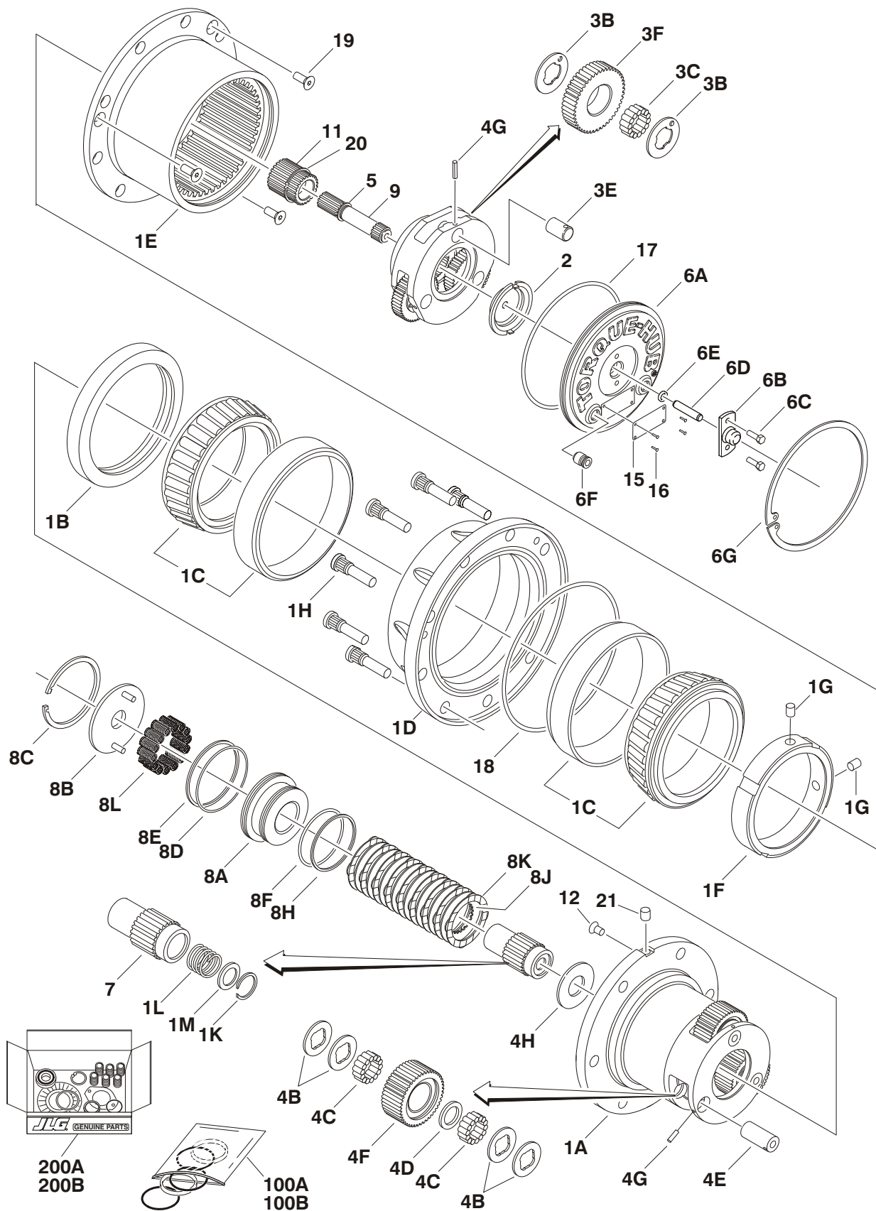
FIGURE 1-7. DRIVE HUB ASSEMBLY (S/N 85132 TO PRESENT)
