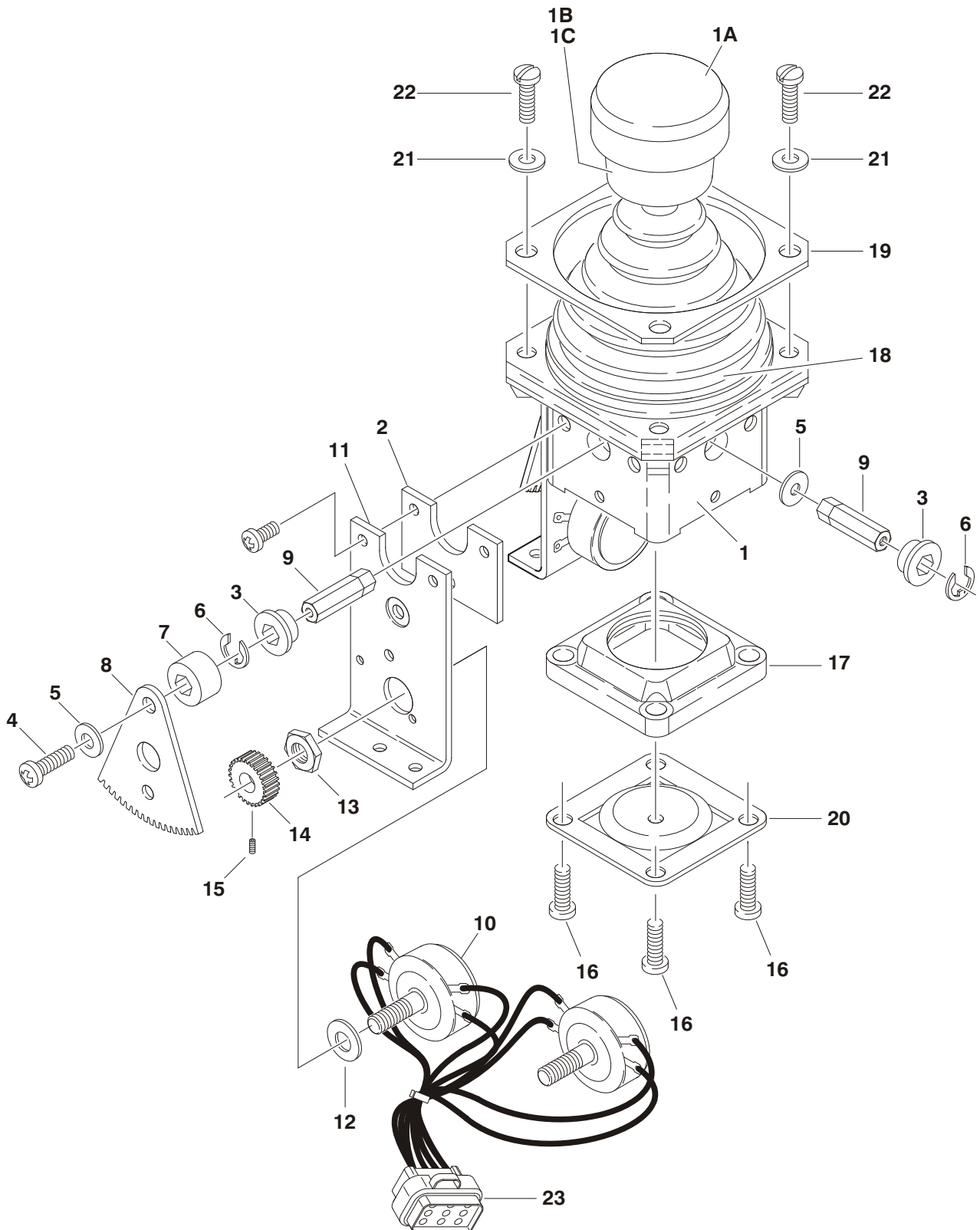
FIGURE 4-7. CONTROLLER ASSEMBLY (SWING & LIFT) (WITHOUT ADE SYSTEM) (S/N 62137 TO PRESENT)
