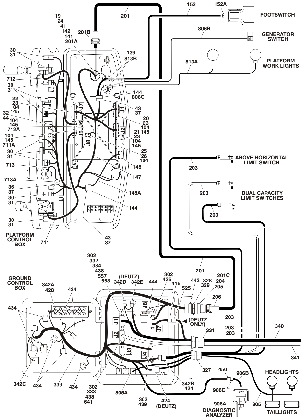
FIGURE 7-10. HARNESS COMPONENTS INSTALLATION (DEUTZ EMR2) (S/N 85132 TO PRESENT)
