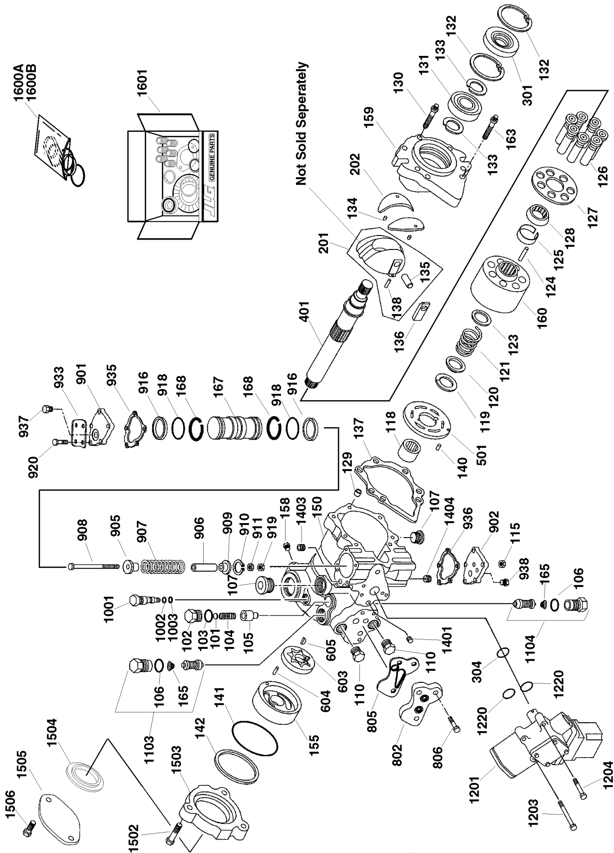
FIGURE 2-20. PISTON PUMP ASSEMBLY (W/HYDRAULIC WELDER)
