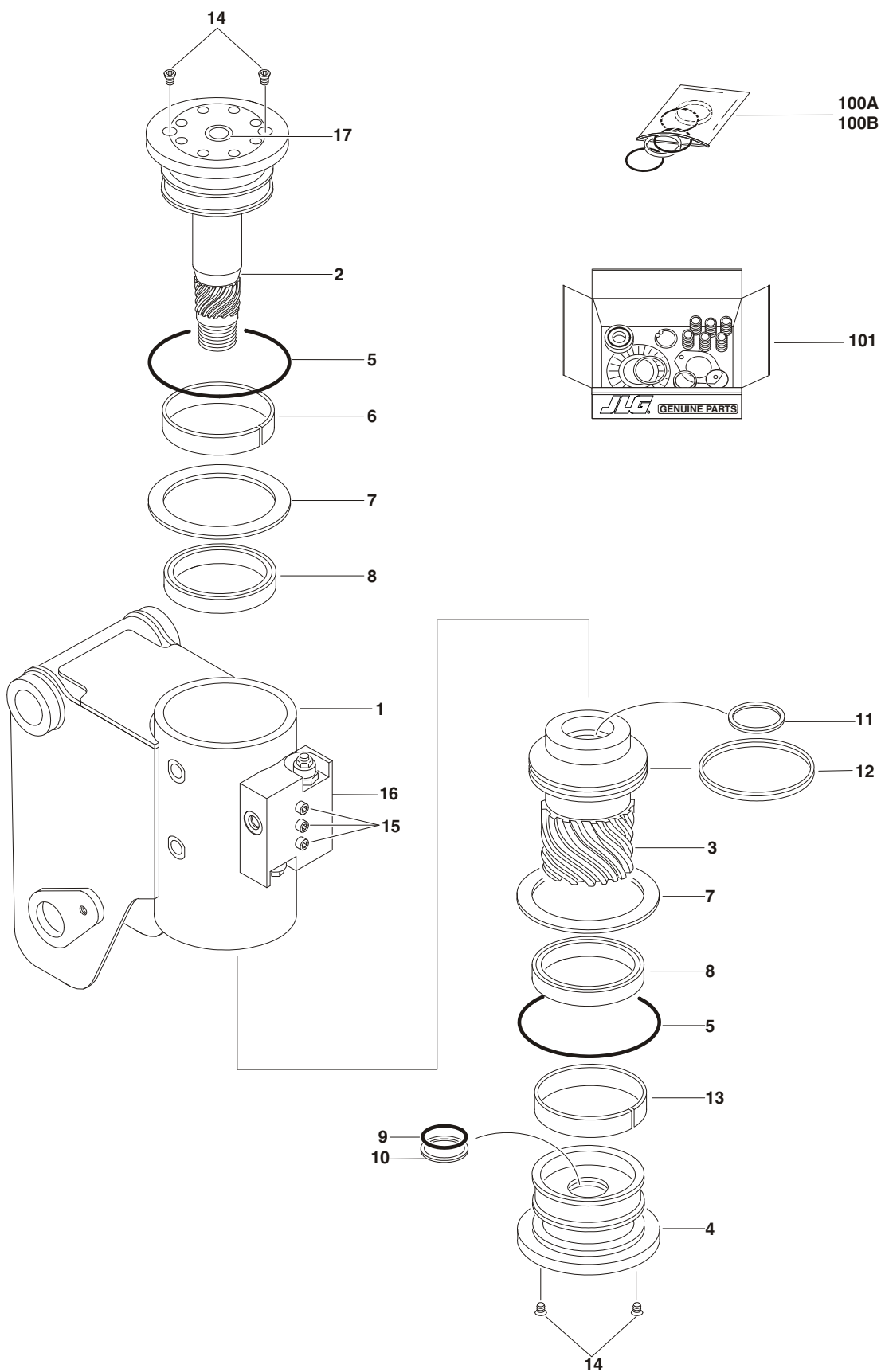
FIGURE 3-4. ROTATOR ASSEMBLY (SIDE ENTRY PLATFORM)
