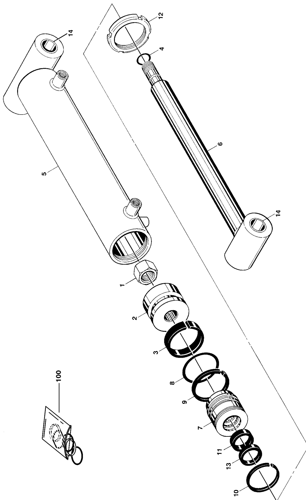
FIGURE 5-6. STEER CYLINDER ASSEMBLY (PRIOR TO S/N 85132)
