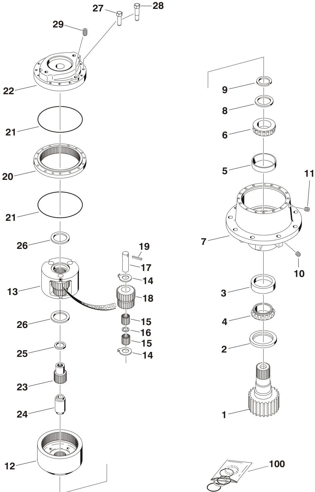
FIGURE 2-6. SWING HUB ASSEMBLY
