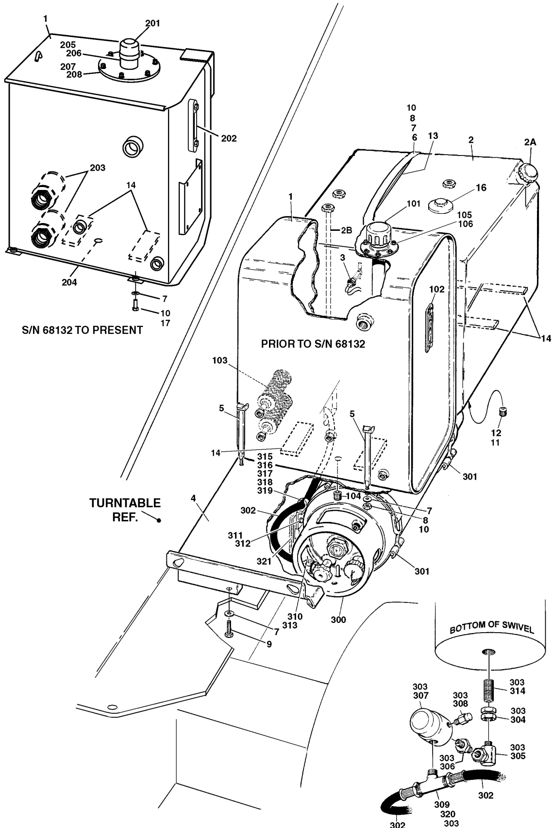
FIGURE 2-23. TANK INSTALLATIONS
