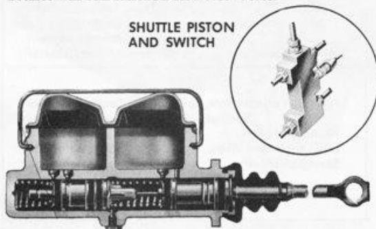
DUAL MASTER CYLINDER
