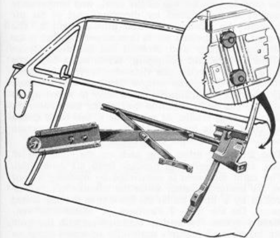
WINDOW REGULATOR AND GUIDE
