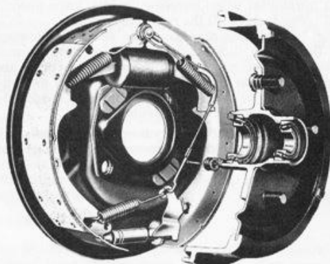
STANDARD DRUM BRAKES
