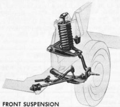
FRONT SUSPENSION
