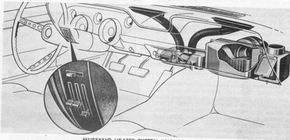
MUSTANG HEATER SYSTEM AND CONTROLS
