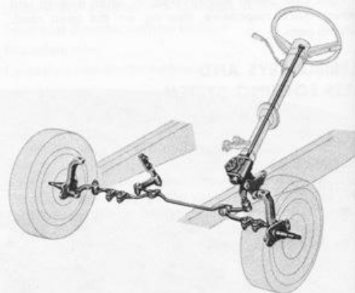
MUSTANG MANUAL STEERING
